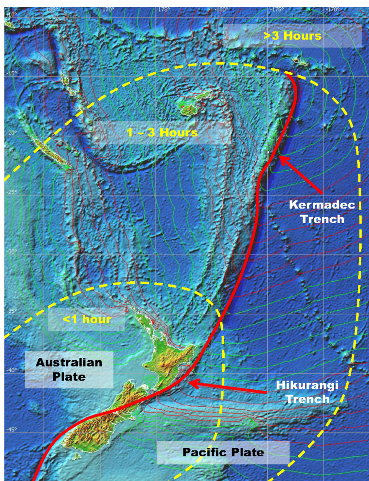
Figure 4: Map showing tsunami arrival times
