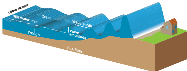
Figure 2: Change in wave length and height as a tsunami approaches the shore
