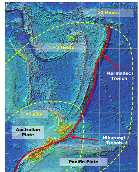
Figure 1: Regional and distant source zones for tsunami impacting New Zealand. Zones are calculated by the distance to nearest part of the New Zealand coast
